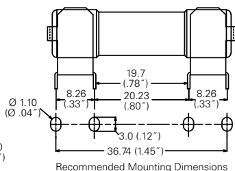
0106 0001 Device Dimensions
