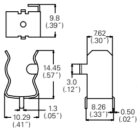
0106 0001 Device Dimensions
