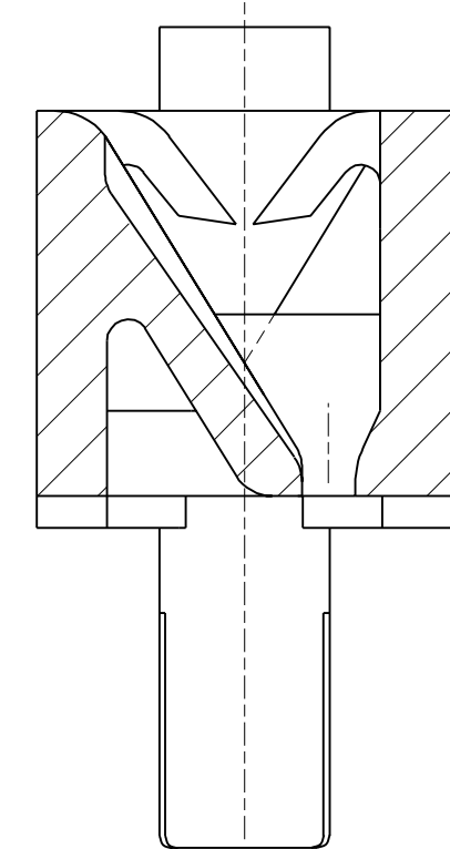
SECTION "D"- "D" ROTATED 90°
