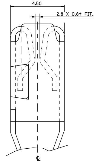
DETAIL D
