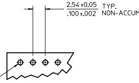
TYP. HOLE PATTERN FOR 1.57/.062 THK. PCB
