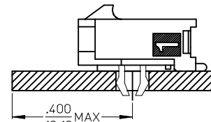
LOCATION DETAIL SEE NOTE #8
