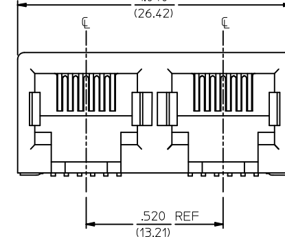
6 CIRCUIT ASSEMBLY
