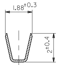
SECT. B-B
