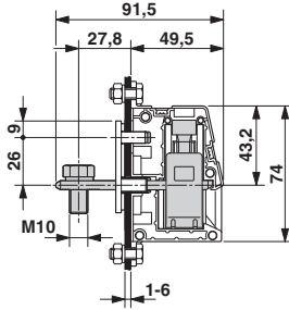
Dimensional drawing
