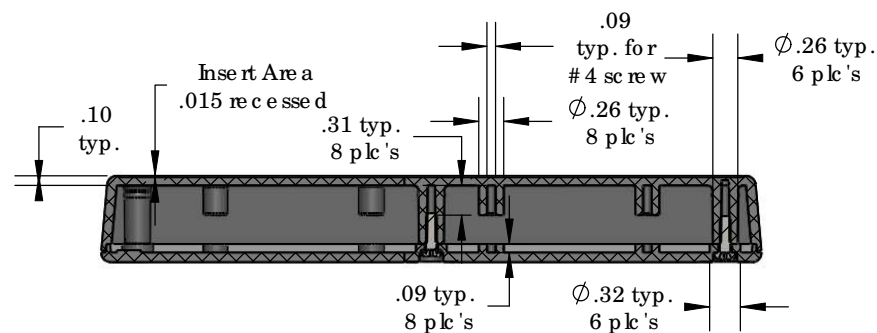
No tes: Enc lo sure we ight .34 lbs /154 gm SECTION A-A 1) Enc lo sure me ets o r ex ce eds IP40 and NEMA 1 SCALE 1 : 2 2) C ir c u it Bo ar d dr aw ing s c a n be do wn lo ad at: http://www.serpac.com/Accessories/CircuitBoard/drawings/370-470.pdf 3) All co m po n e n t s a r e R o H S Co m p l i a n t .
