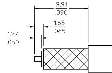
RECOMMENDED CABLE STRIP DIMENSIONS
