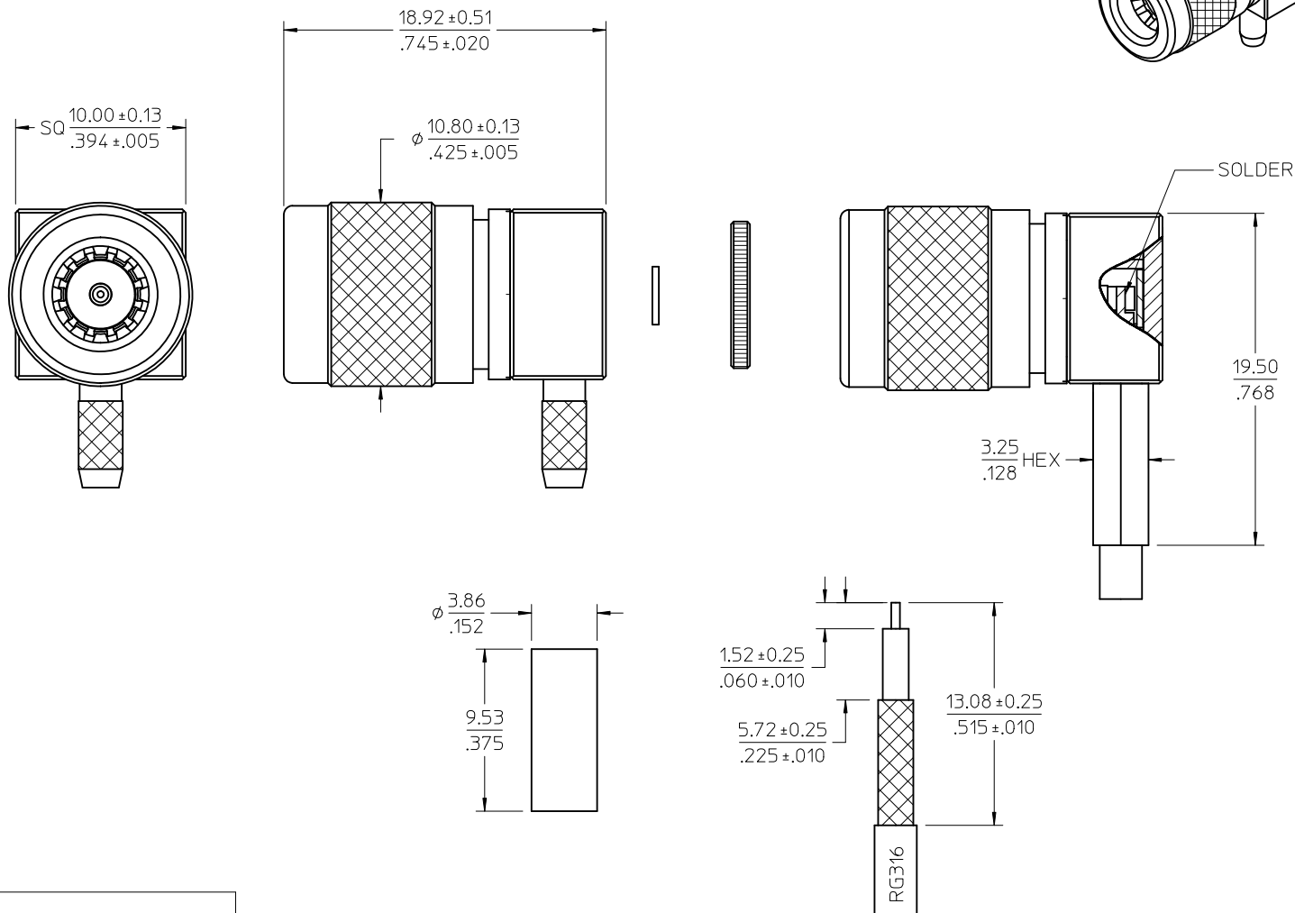
STRIPPING DIMENSIONS
