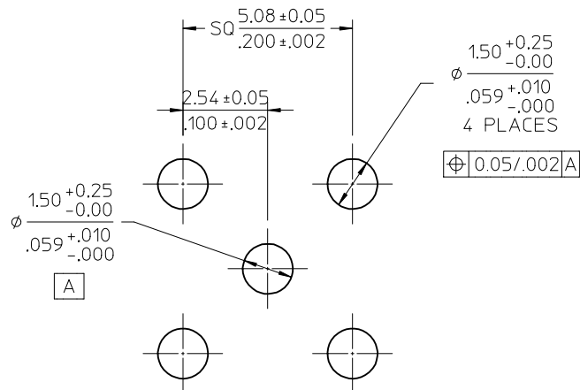
RECOMMENDED PCB CONFIGURATION
