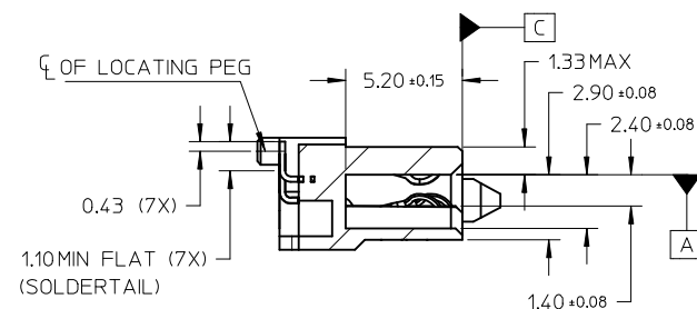
SECTION Z-Z
