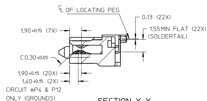
SECTION Y-Y
