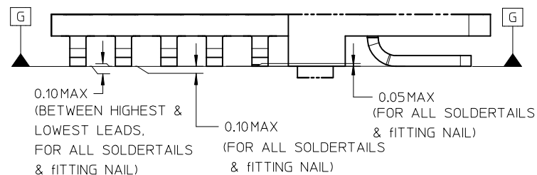
DETAIL1
