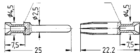
Identification of the crimp contacts
