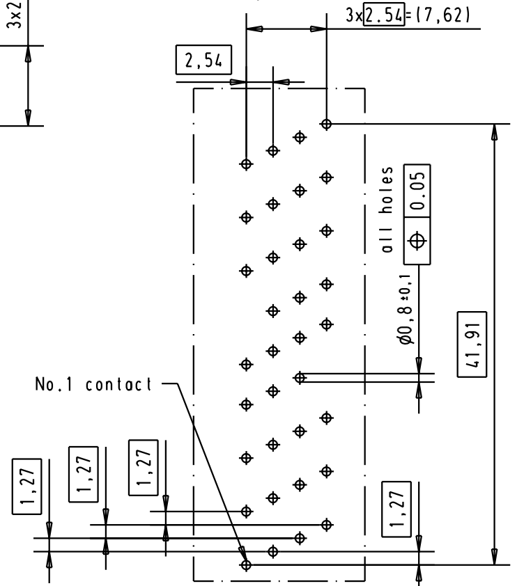
Printed board layout Component side
