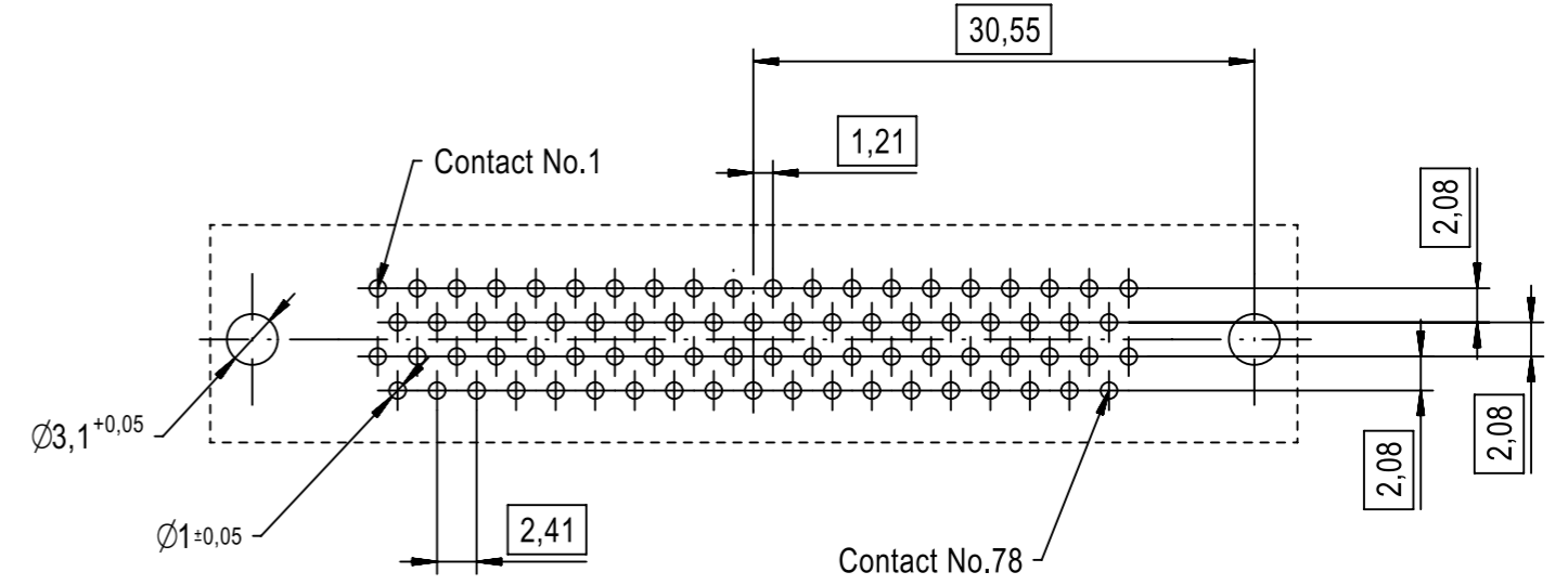
PC-Board layout view component side thickness 1,6 mm
