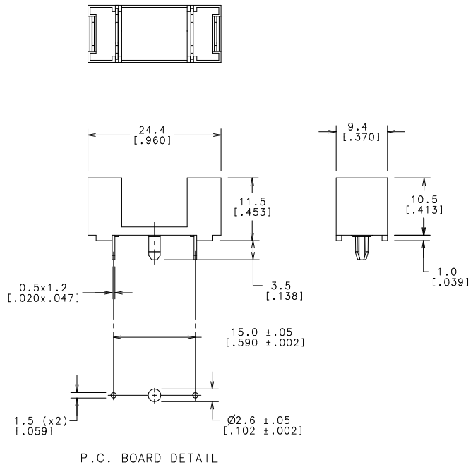
P.C. BOARD DETAIL
