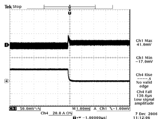
Vout=1.8 V 50%-0% Load Transients
