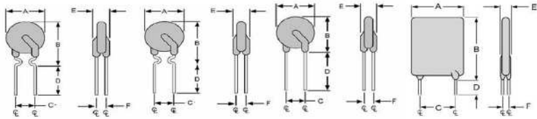
Fig.1 Lead Size : 24AWG \Phi 0.51 mm Diameter Fig.2 Lead Size : 22AWG \Phi 0.65 mm Diameter Fig.3 Lead Size : 20AWG \Phi 0.81 mm Diameter Fig.4 Lead Size : 20AWG \Phi 0.81 mm Diameter
