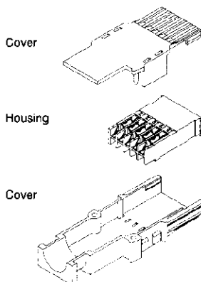
10 Positions, Unshielded
