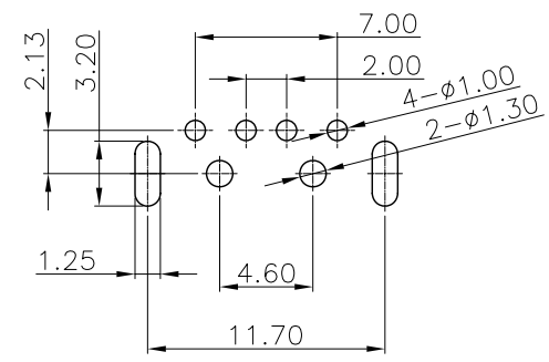
RECOMMENDED P.C.B. PATTERN LAYOUT
