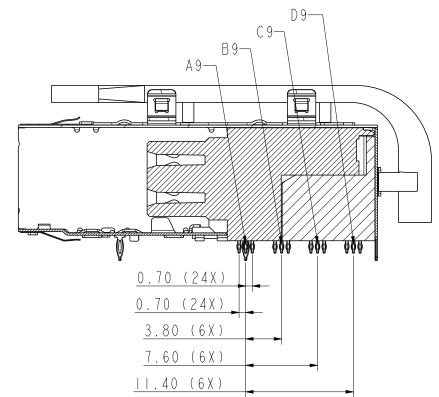
SECTION Z-Z
