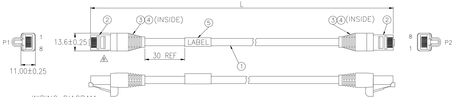
WIRING DIAGRAM
