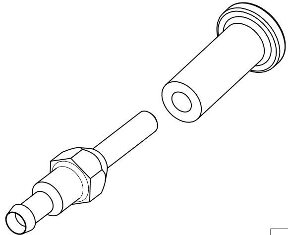
ISOMETRIC VIEW SCALE 8:1
