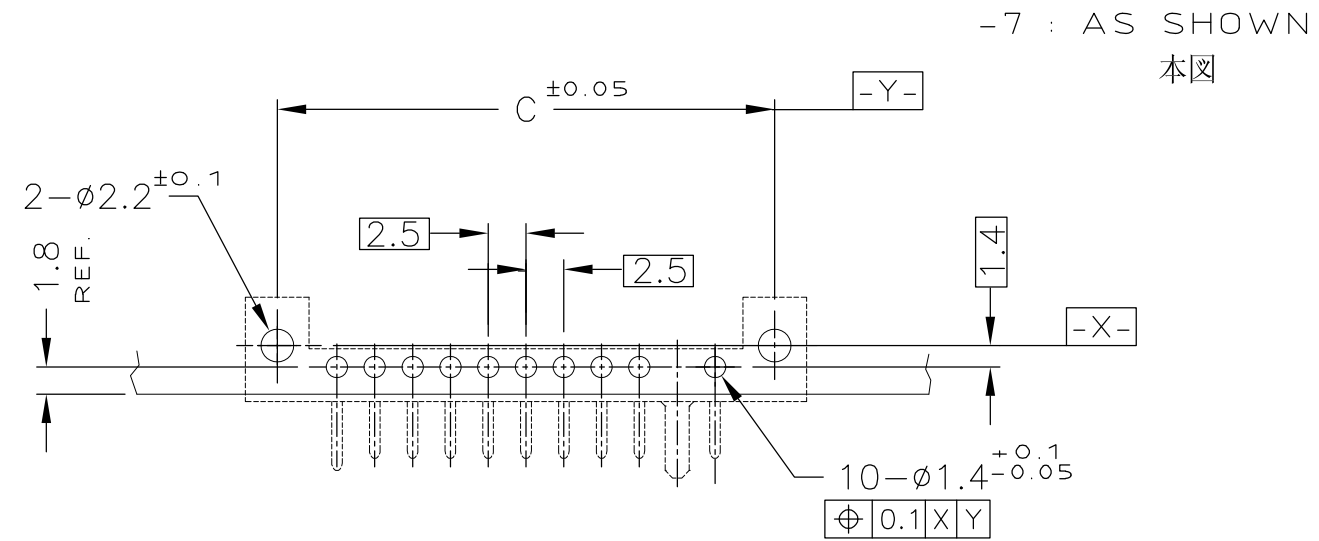
基板取付推奨寸法 RECOMMENDED P.C. BOARD LAYOUT P.C. BOARD THK 0.8~1.2 (VIEW FROM CONNECTOR MOUNTING SIDE)
