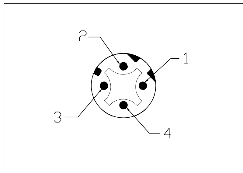
FRONT VIEW - MALE INSERT
