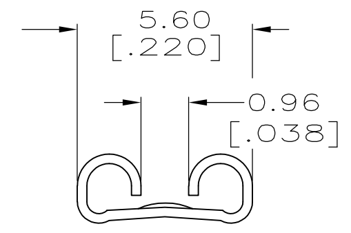
VIEW A-A SCALE 6:1
