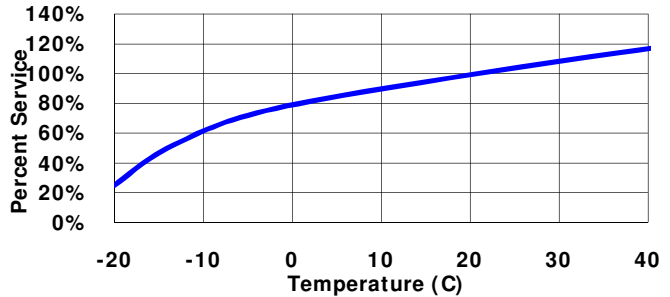
TYPICAL PERCENT SERVICE 3.9 ohm - 4 hours/ day to 0.75 volts
