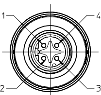
MALE FACE VIEW SCALE 2:1
