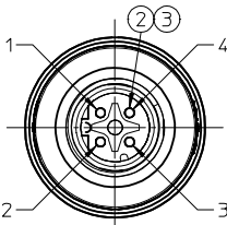
MALE FACE VIEW SCALE 2:1
