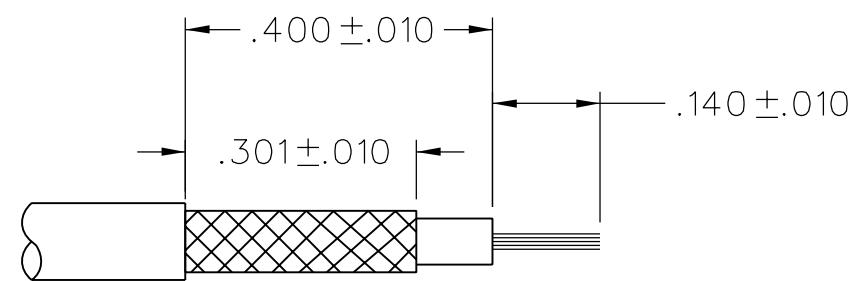
CABLE STRIP DIMENSIONS
