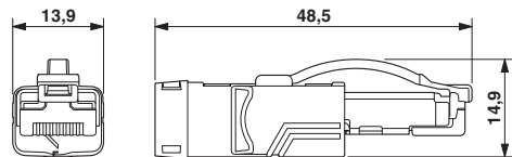
RJ45 plug connector, IP20
