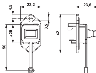
Sealing plug for push-pull panel mounting frame
