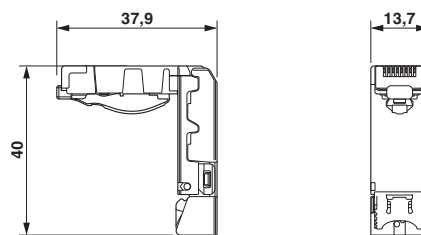
Dimensional drawing
