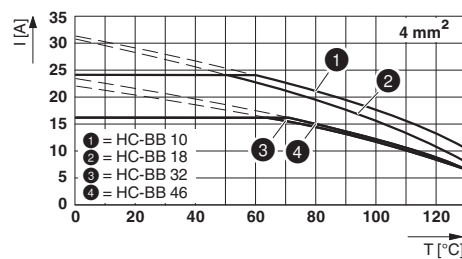
Derating diagram (conductor cross section: 4.0 mm²)
