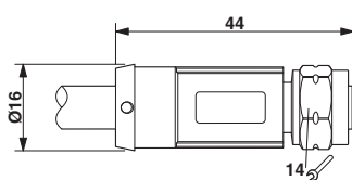
Dimensional drawing
