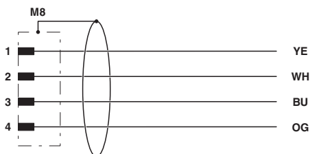
Contact assignment of the M8 plug
