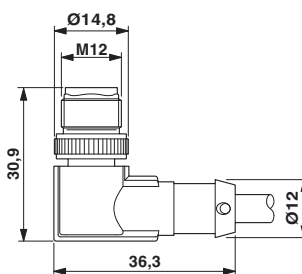
M12 x 1 male plug, angled, shielded
