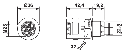
Dimensional drawing
