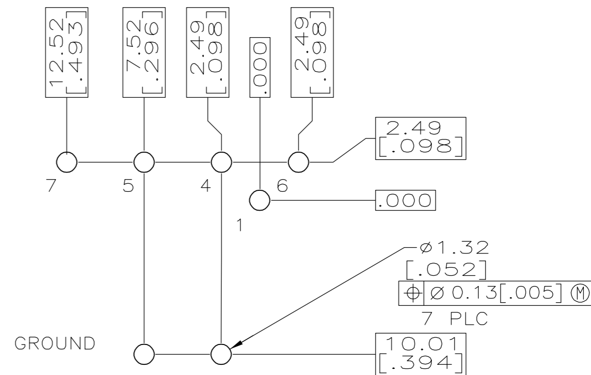
SUGGESTED PC BOARD LAYOUT & CIRCUIT IDENTIFICATION
