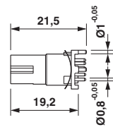
Dimensional drawing
