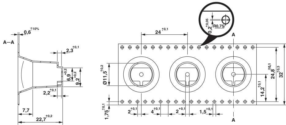
Dimensional drawing
