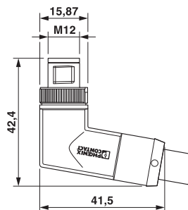
Dimensional drawing
