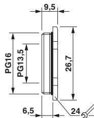
Dimensional drawing
