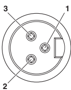
Pin assignment, socket, 7/8"-16UNF, 3-pos., view of female side
