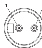
Pin assignment, plug, 7/8"-16UNF, 2-pos., view of male side
