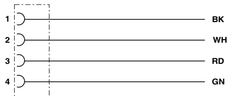
Contact assignment of 7/8" socket
