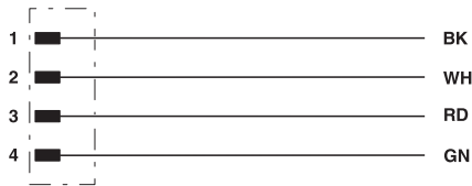
Contact assignment of the 7/8" plug
