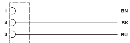
Contact assignment of the M12 socket
