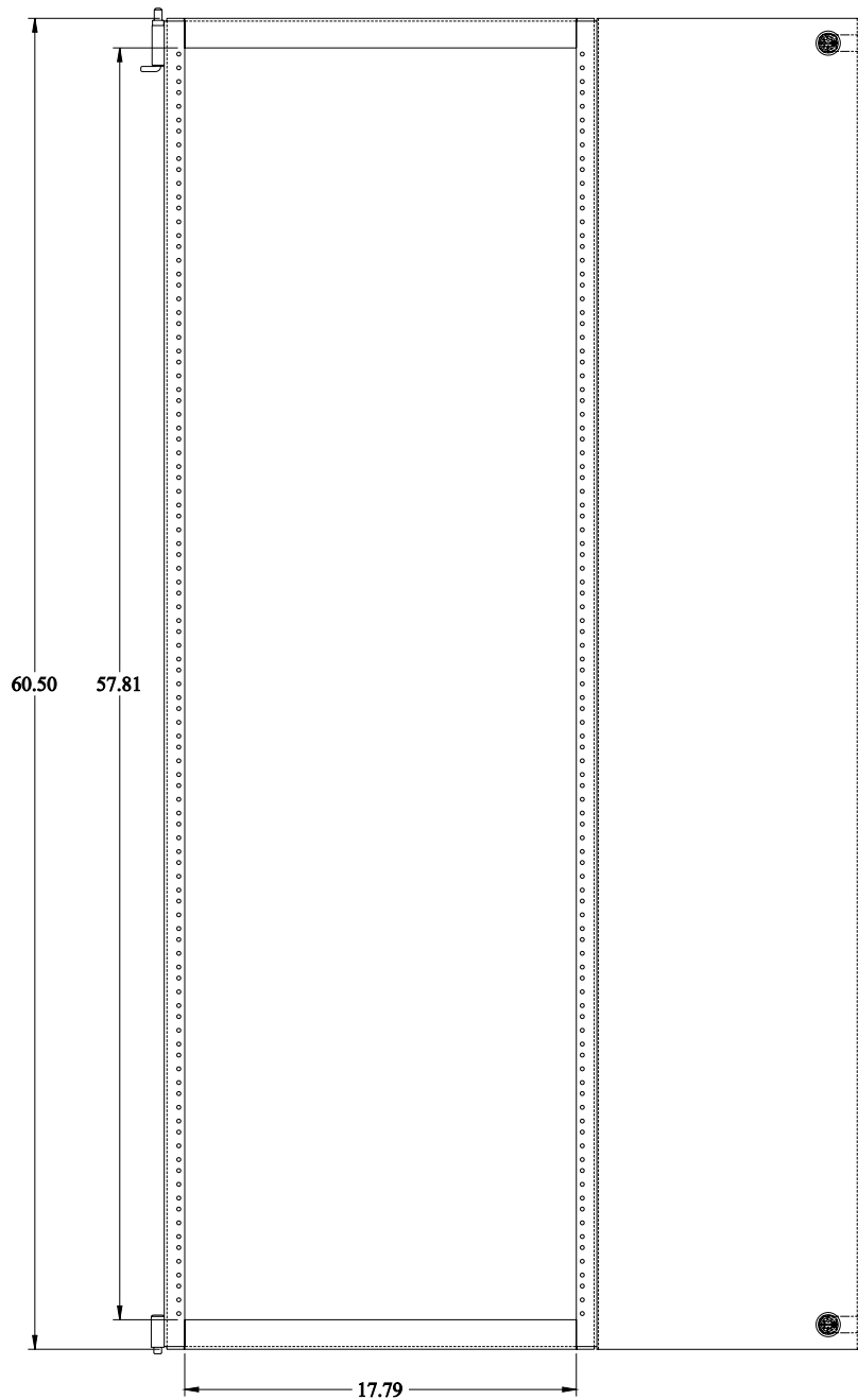
FRONT VIEW
