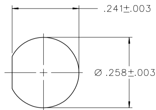
MOUNTING HOLE 4:1
