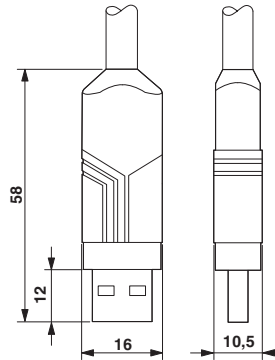
Dimensional drawing
